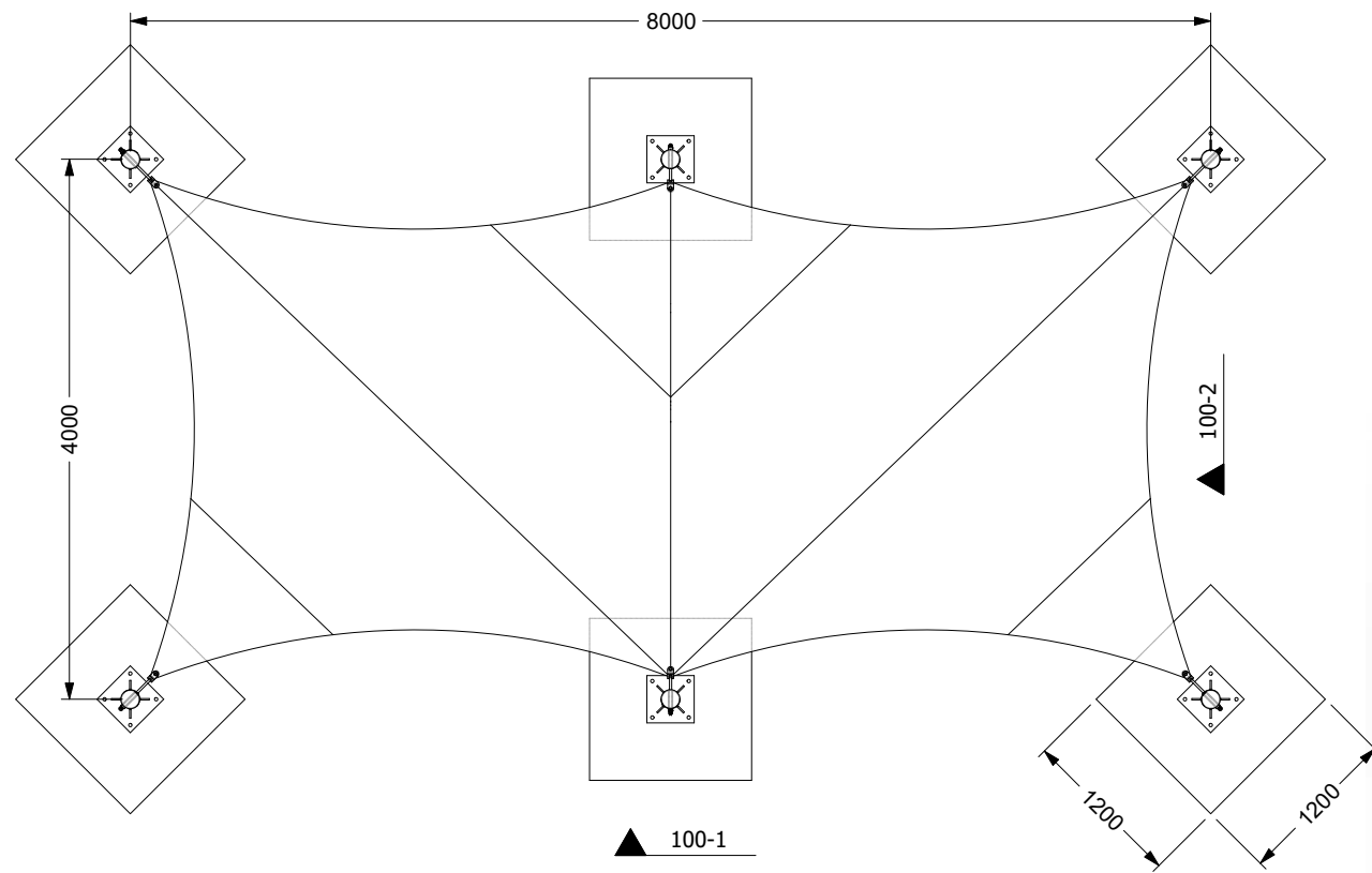
PLAN SCALE 1:60 @ A3
