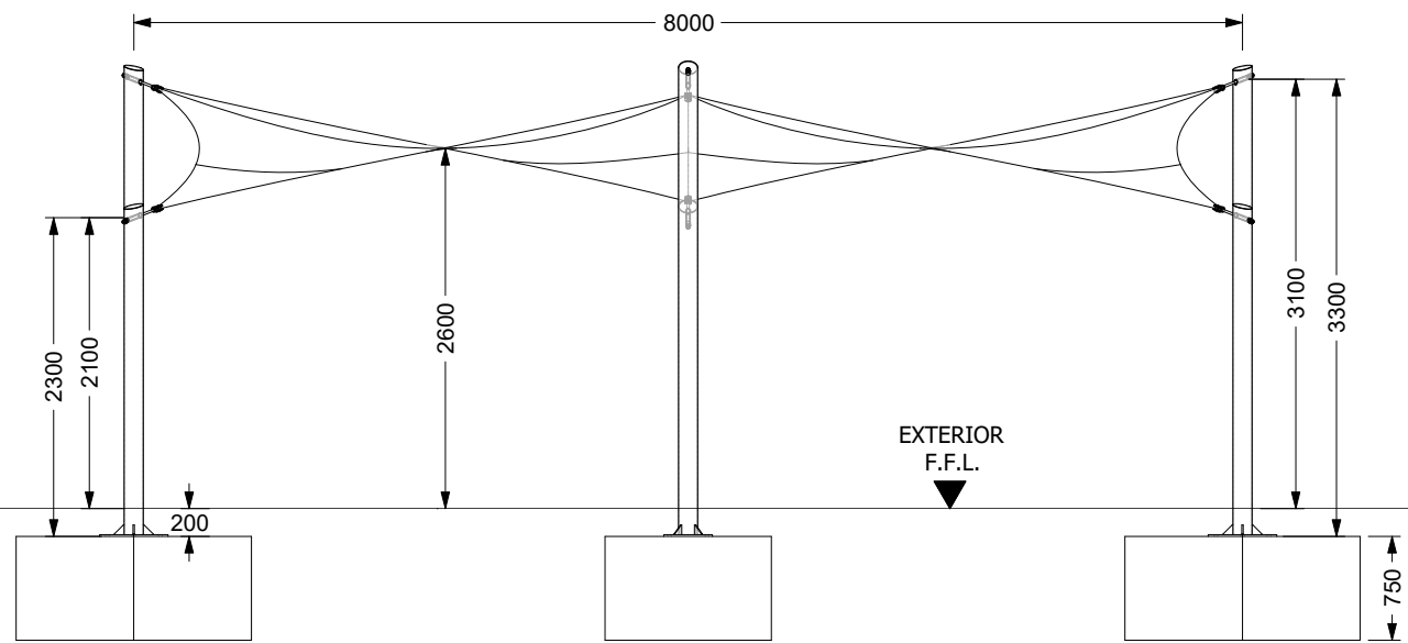
100-1 ELEVATION SCALE 1:60 @ A3
