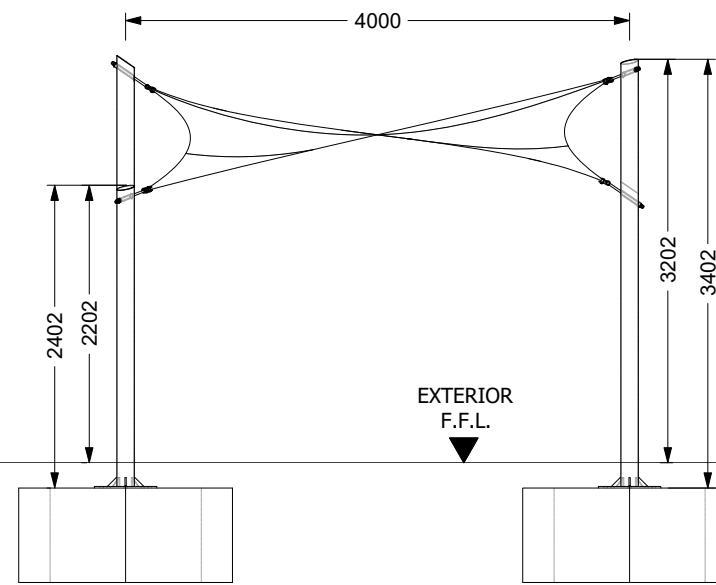
100-2 ELEVATION SCALE 1:60 @ A3
