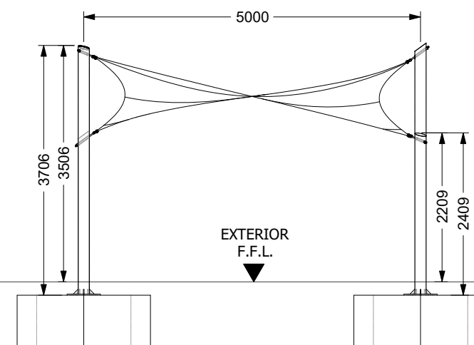
100-2 ELEVATION SCALE 1:80 @ A3
