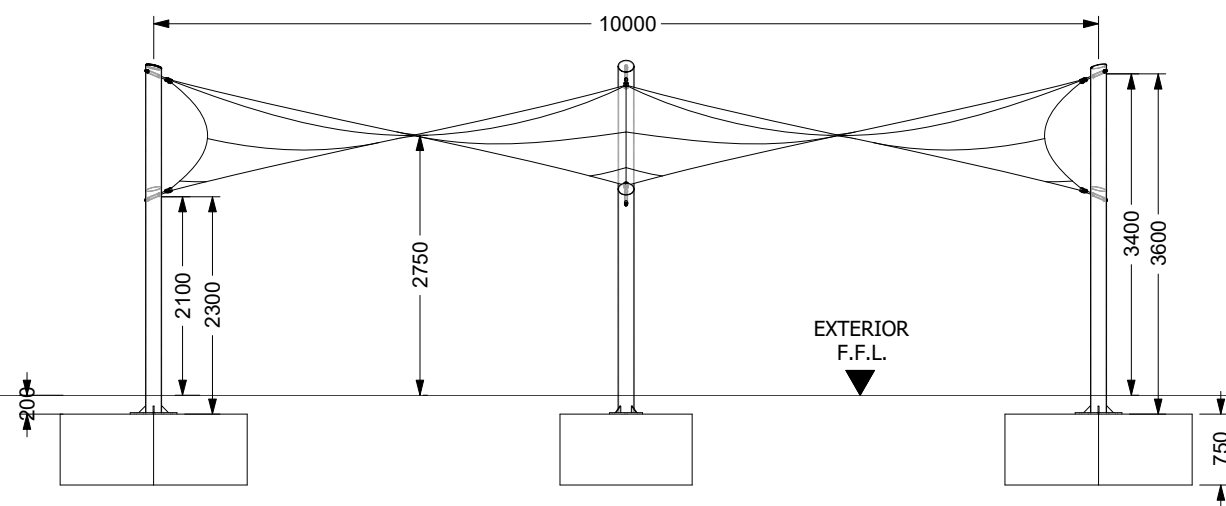
100-1 ELEVATION SCALE 1:80 @ A3
