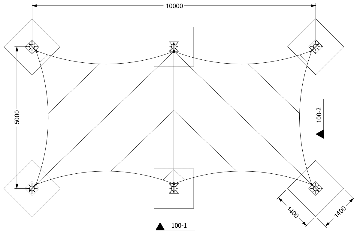
PLAN SCALE 1:80 @ A3
